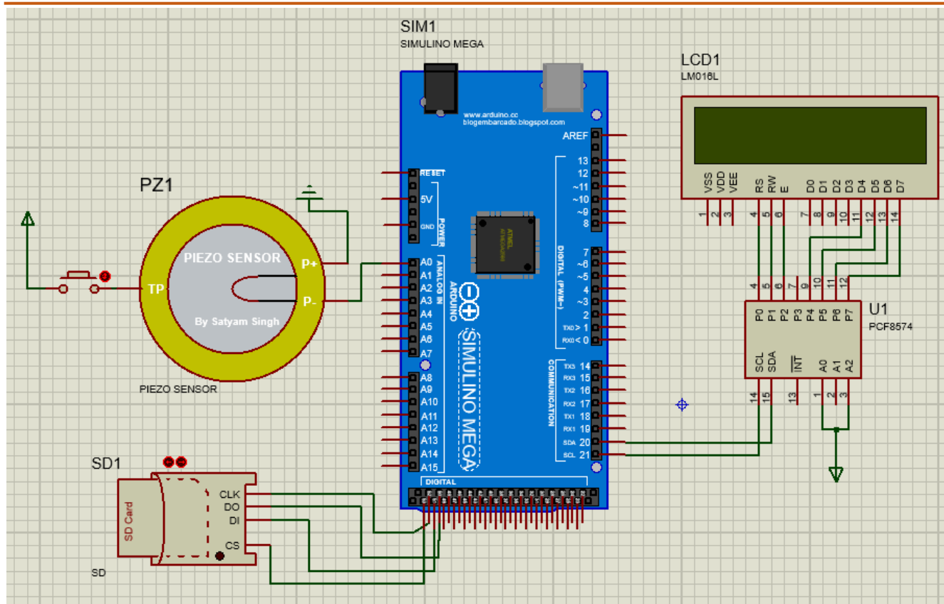
Figure 8. Instrumentation system circuit in Proteus.
