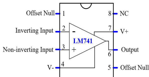
Figure 11. LM741 pinout diagram
