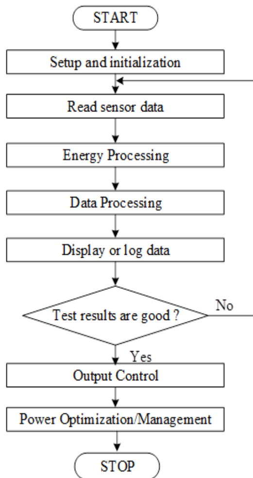
Figure 7. Flow diagram for designing Arduino software for piezoelectric energy harvesters
