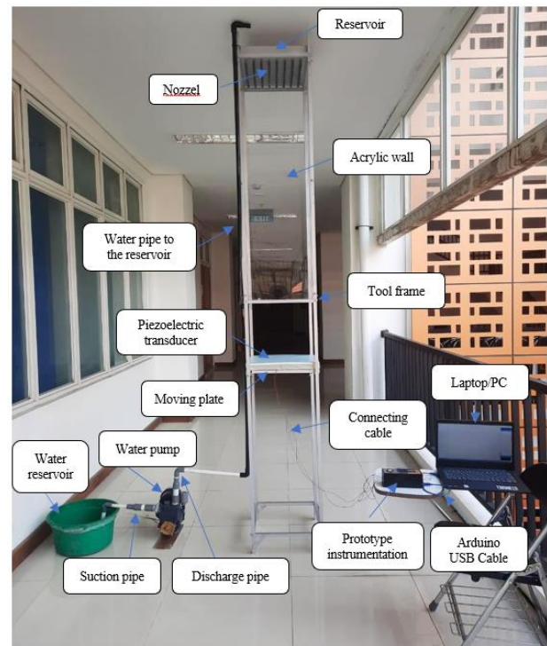
Figure 15. Experimental setup for data collection
